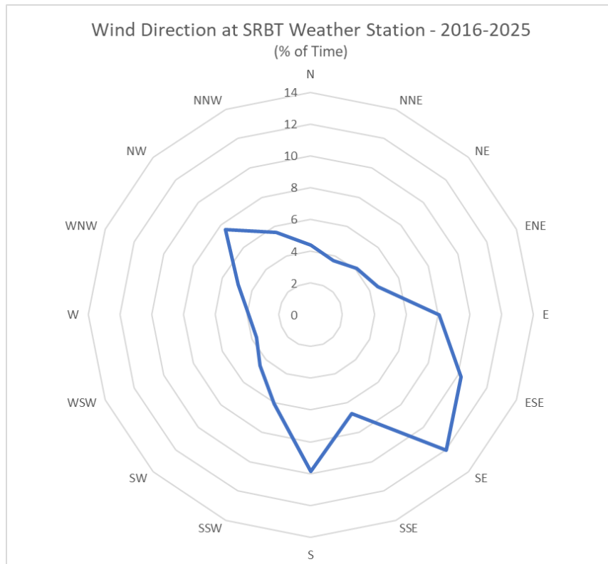
FIGURE 7: WIND DIRECTION DISTRIBUTION WINDROSE (2016-2025)
